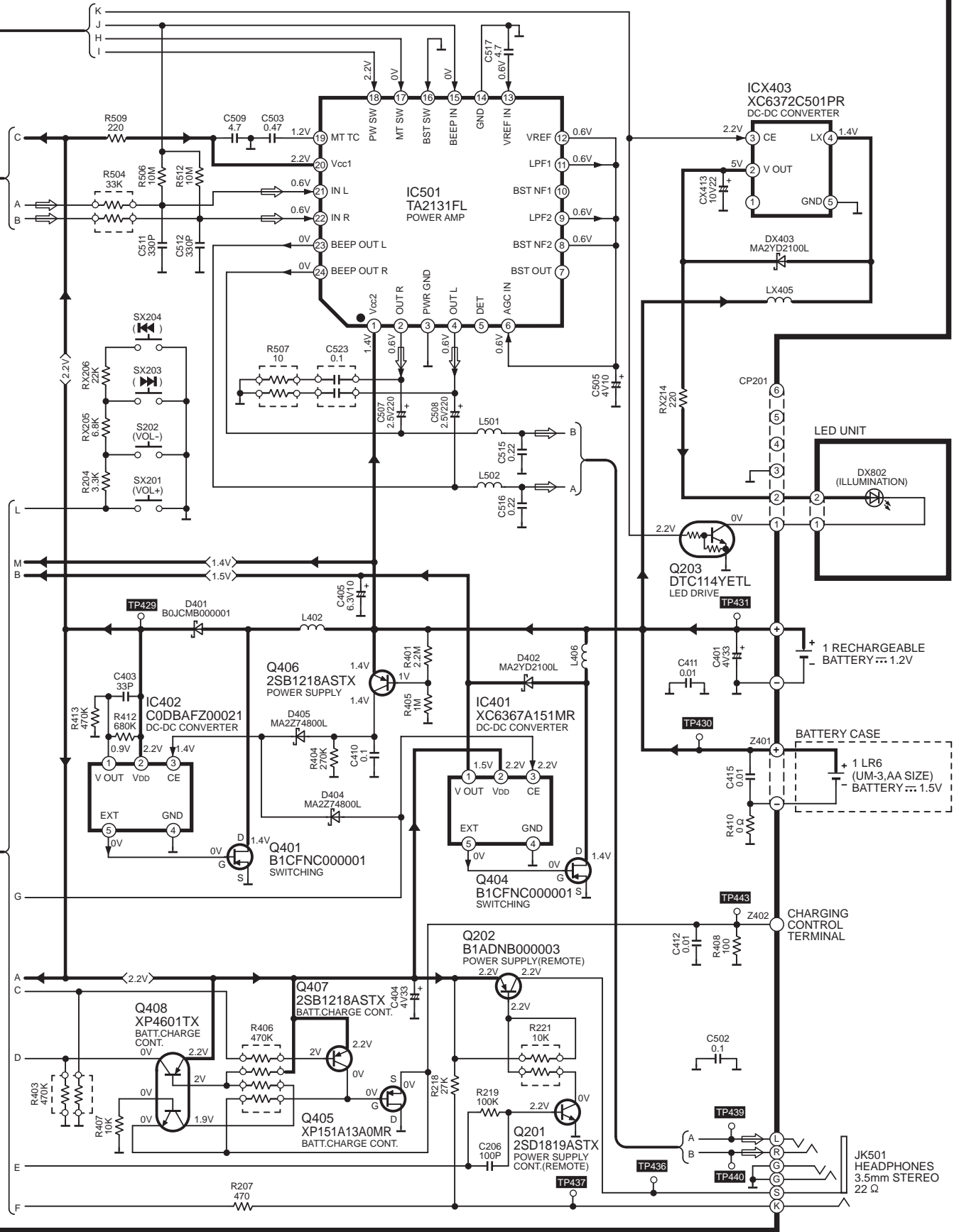
SJ-MJ50(GH) CIRCUIT DIAGRAM
